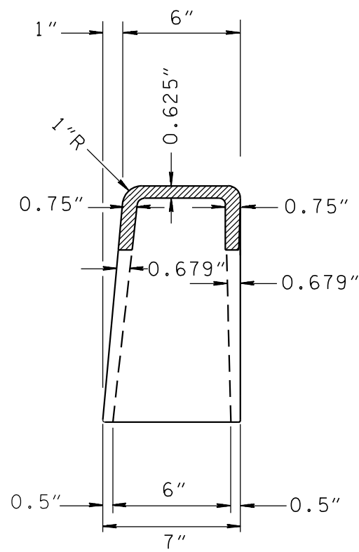
SECTION E-E
