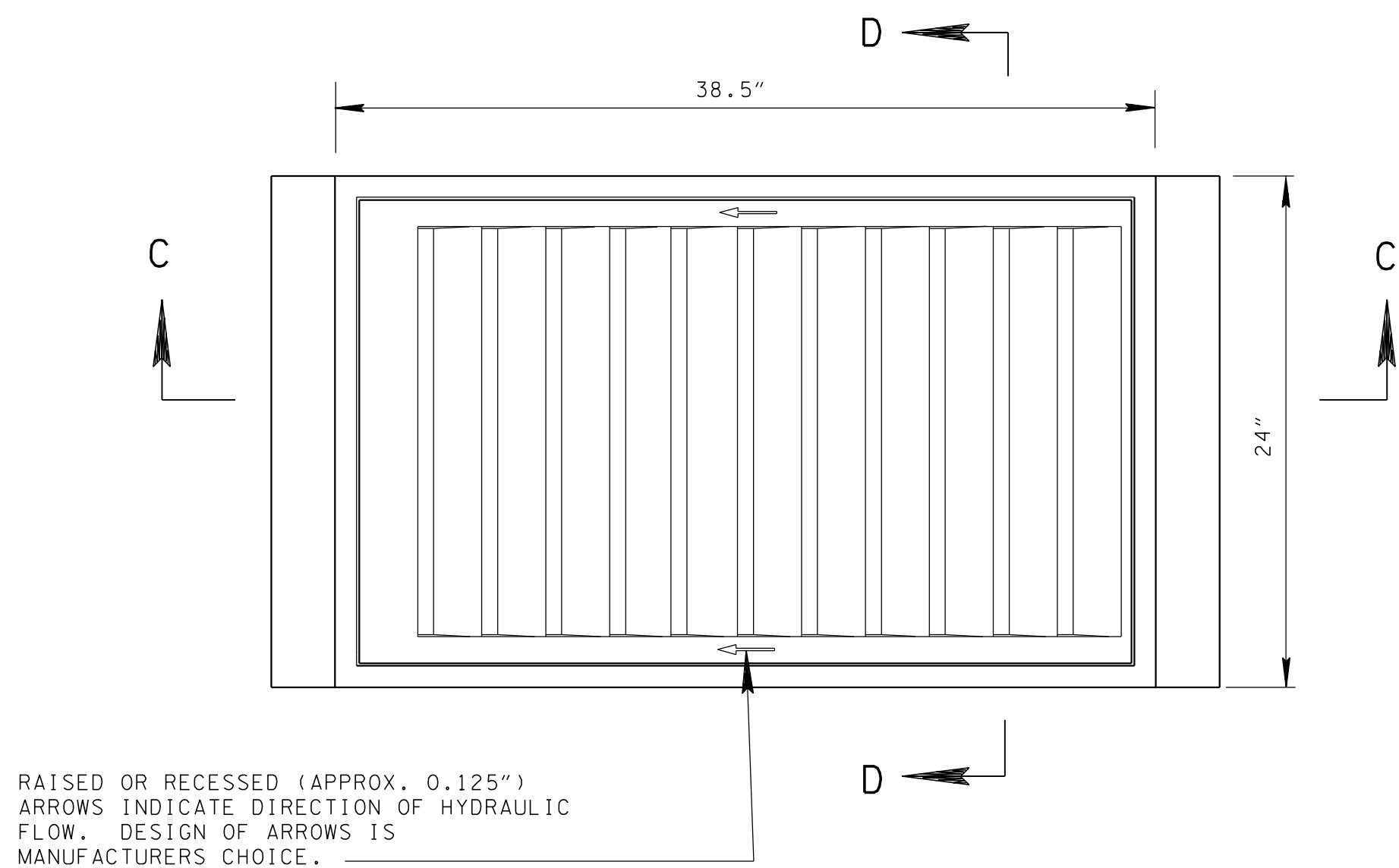
PLAN VIEW
